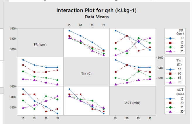
Figure 16. Interaction plot for X*
