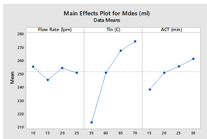
Figure 6. Mean plot for M_{des} with 3 factors at 4 level
