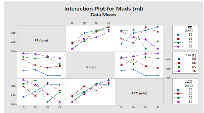
Figure 15. Interaction plot for M ads
