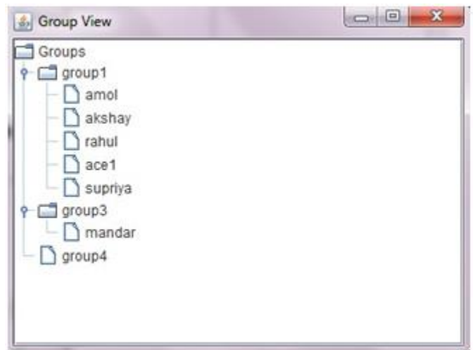
Figure 16: View group
