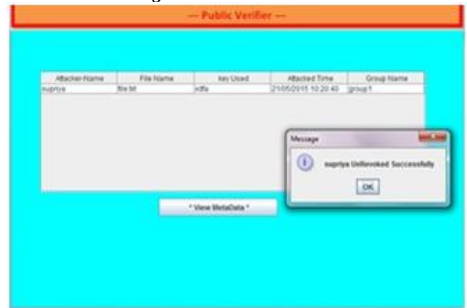
Figure 14: User unrevoked
