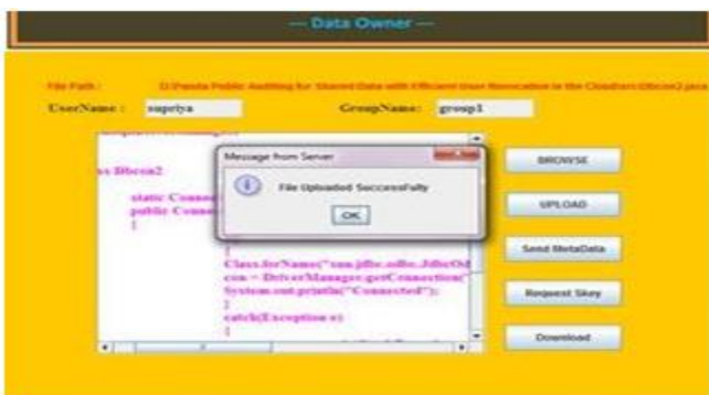
Figure 7: Upload file
