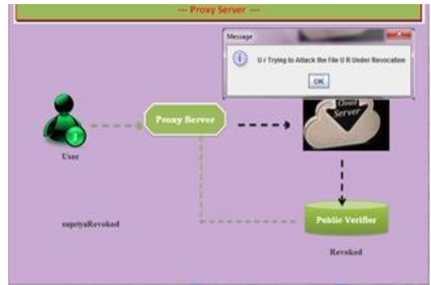
Figure 12: View metadata
